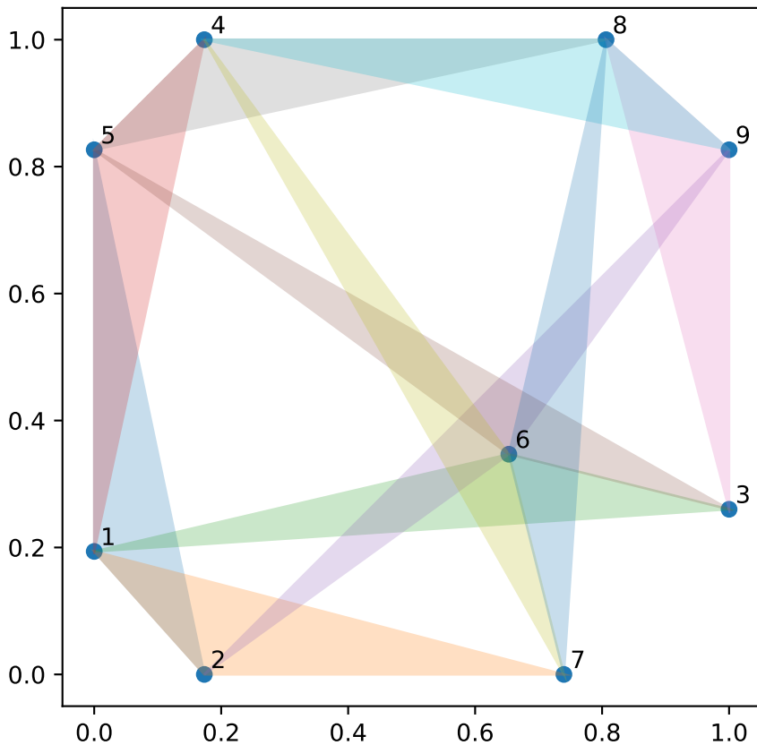
The 11 minimal area triangles for n=9
